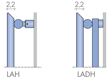
Top and side edges of the panels
