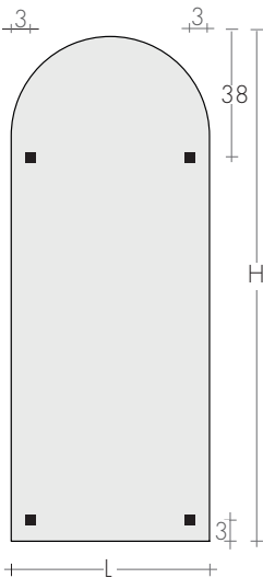
Fitting \varnothing 3/8" STANDARD (without sleeves)
