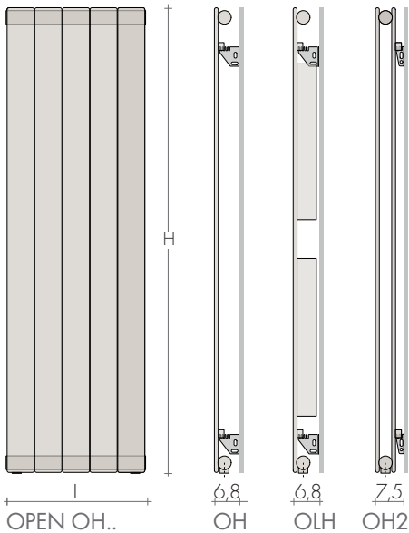
OH Vertical plate and horizontal manifolds
