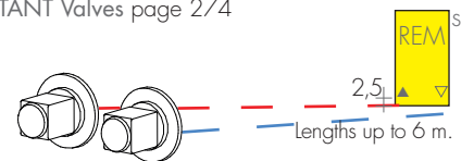
SPECIAL FINISHES page 267 Finishes Gold, Bronze, Brushed Nickel for 2 valves Brushed Nickel FITTING KIT extra Art. RN 30,50€ REMOTE FITTINGS Art. REM 42,10€ Tapping centres: at the rear of radiator \blacktriangle \blacktriangledown 15 cm DISTANT Valves page 274
