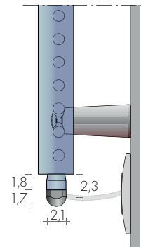
Art. R...II with cable for Wireless Thermostat
