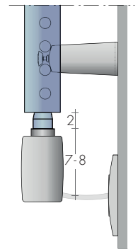
Art. R...IIF \varnothing 1/2 , with Faston for Digital Thermostat
