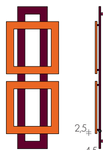
CROSS 152-56 168-64
