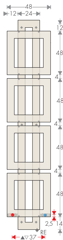
CROSS-Q 230-48
