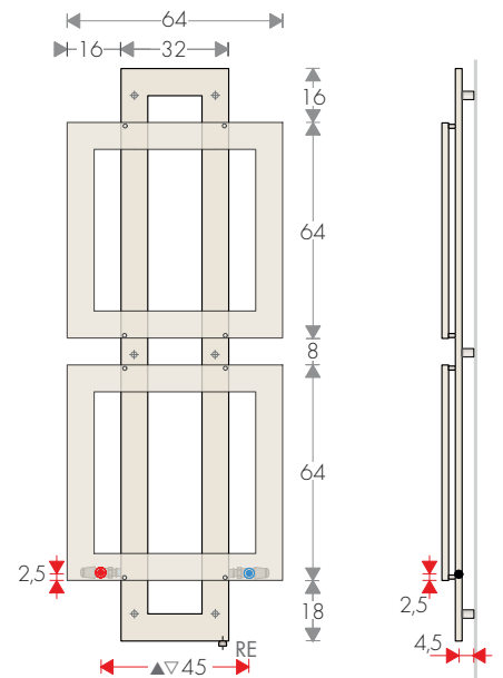
CROSS-Q 170-64
