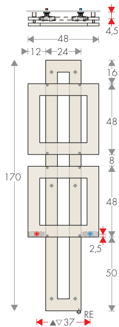
CROSS-Q 170-48
