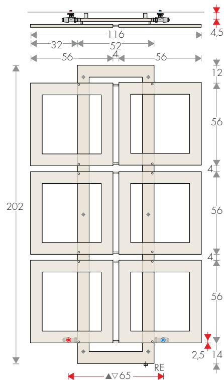
CROSS-Q 202-116
