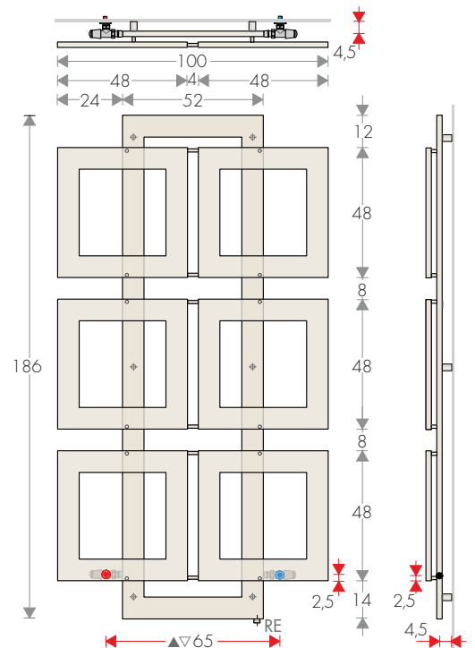
CROSS-Q 186-100
