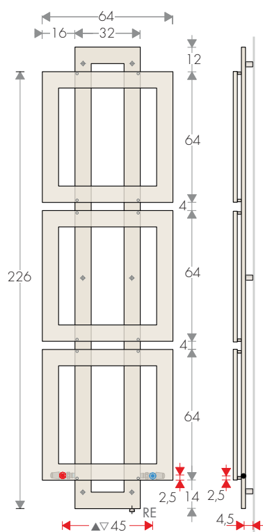
CROSS-Q 226-64
