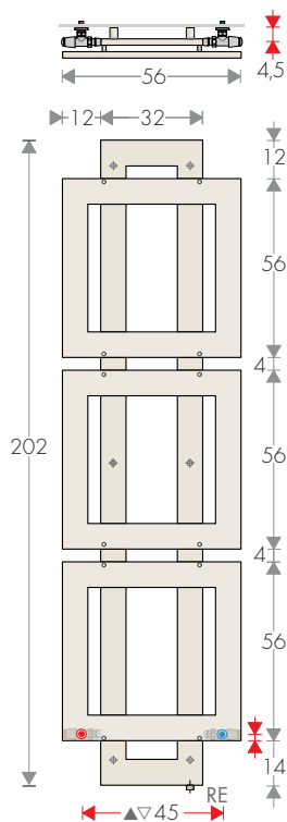
CROSS-Q 202-56
