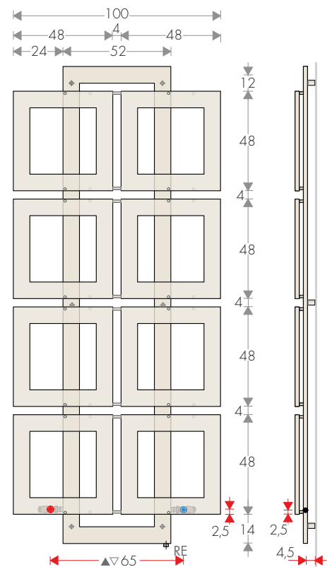
CROSS-Q 230-100
