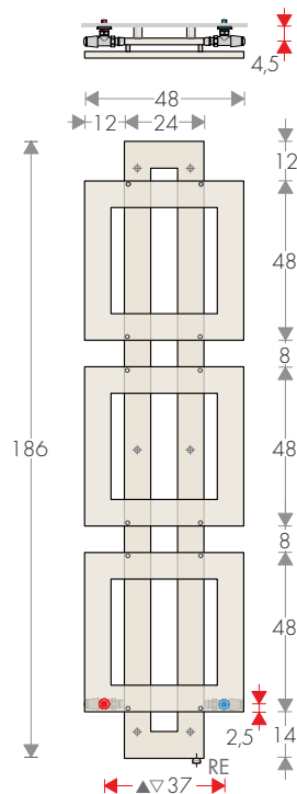
CROSS-Q 186-48
