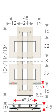
CROSS-RV ...-48
