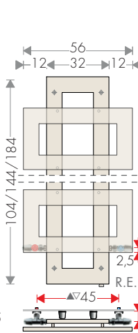
CROSS-RV ...-56
