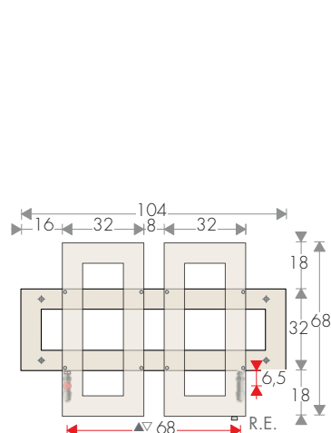
CROSS-RV 68-104
