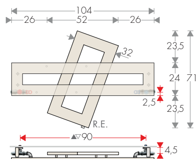
CROSS-R 70-104
