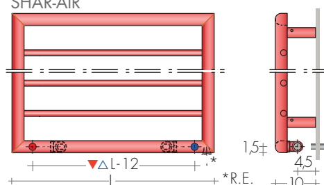
SHAR-A2R
